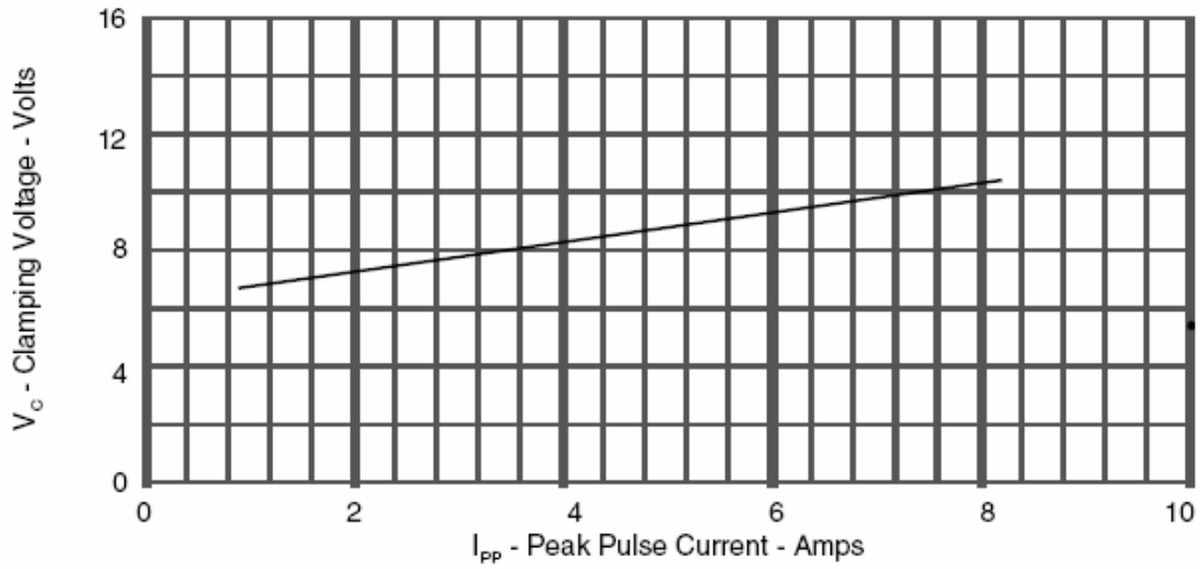
Figure 4 Typical Clamping Voltage VS Peak Pulse Current RSDFS05C
